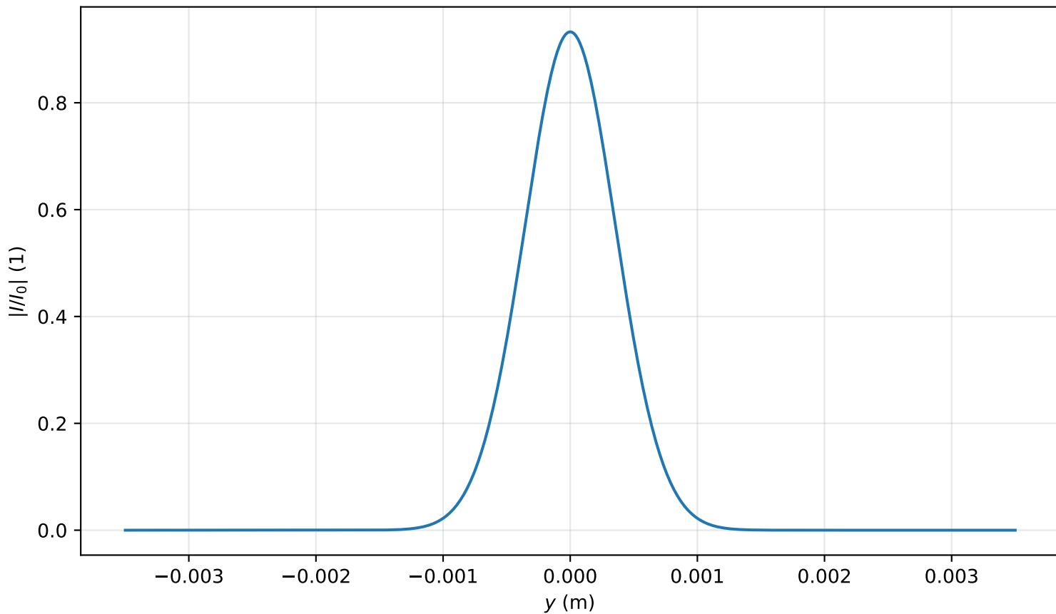
Intensity profile I(x=0, y, z=0.637)/I_0 , \text{Pin}=0.1\text{Pcr} , artificial time
